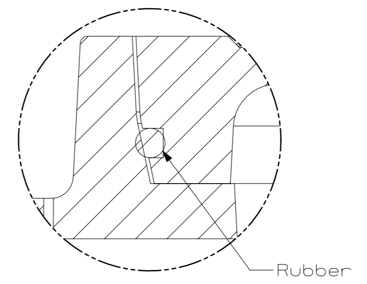
DETAIL F SCALE 1 : 1
